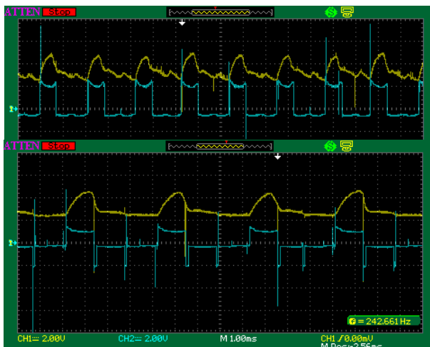
Fig. 25: Test results of the SRM drive in magnetizing and freewheeling modes (a) phase current (b) phase voltage (c) (pulse number on: 0, pulse number off: 500).
